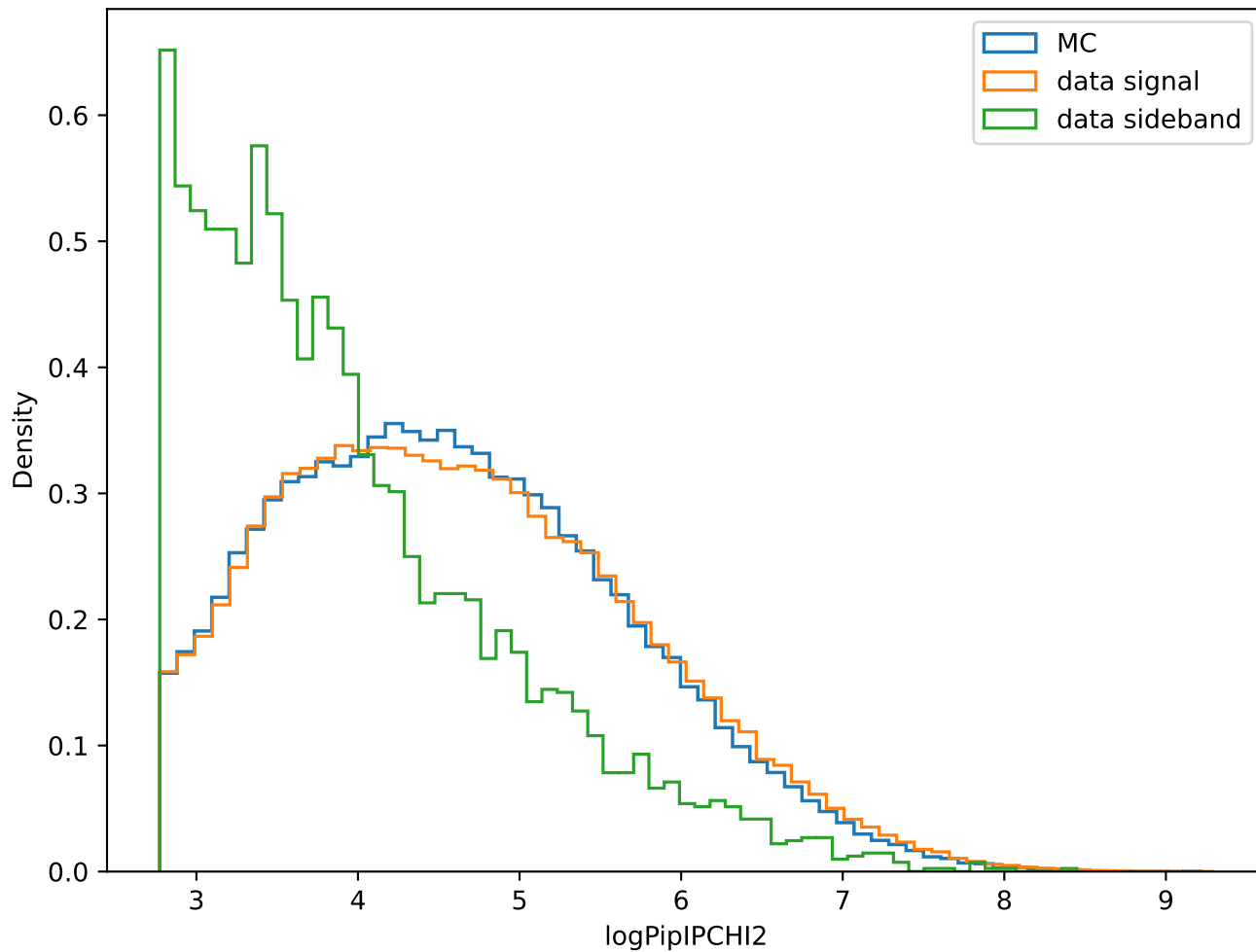
Branch: logPipIPCHI2
