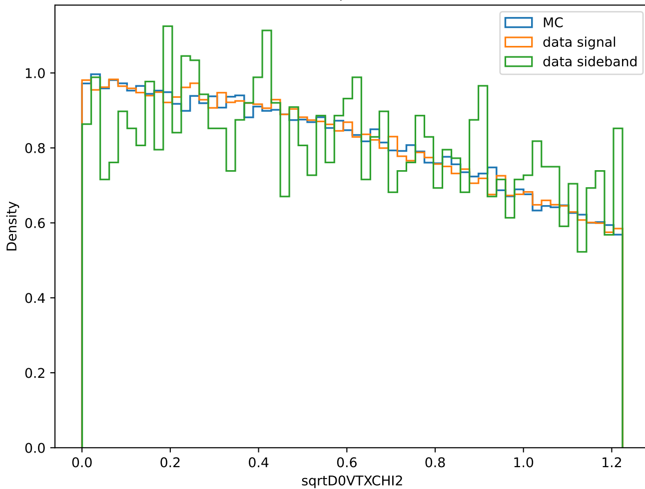
Branch: sqrtD0VTXCHI2
