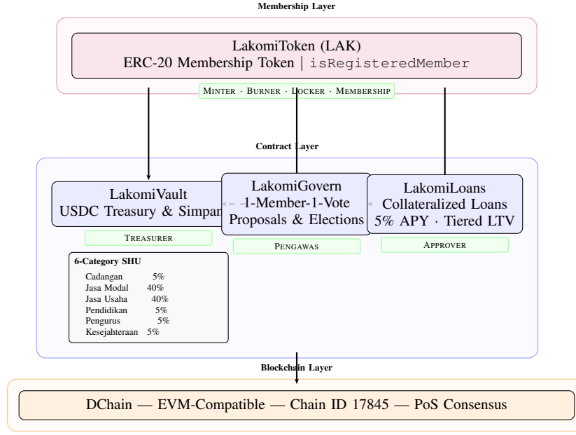
Fig. 1. Lakomi system architecture. LakomiToken serves as the membership registry. LakomiVault manages simpanan and 6-category SHU distribution. LakomiGovern handles proposals, elections, and pengawas veto. LakomiLoans provides collateralized microloans. All contracts execute on DChain.
