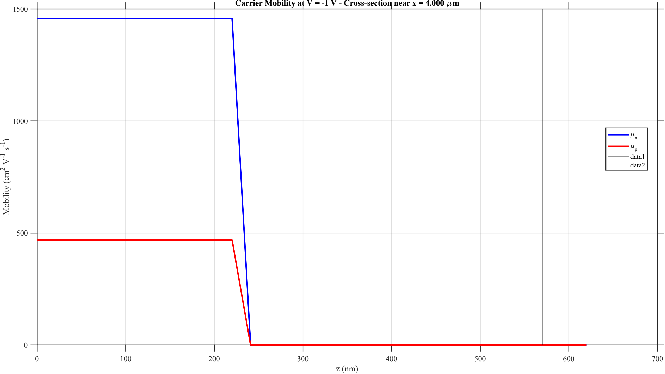
Carrier Mobility at V = -1 V - Cross-section near x = 4.000 \mu\text{m}
