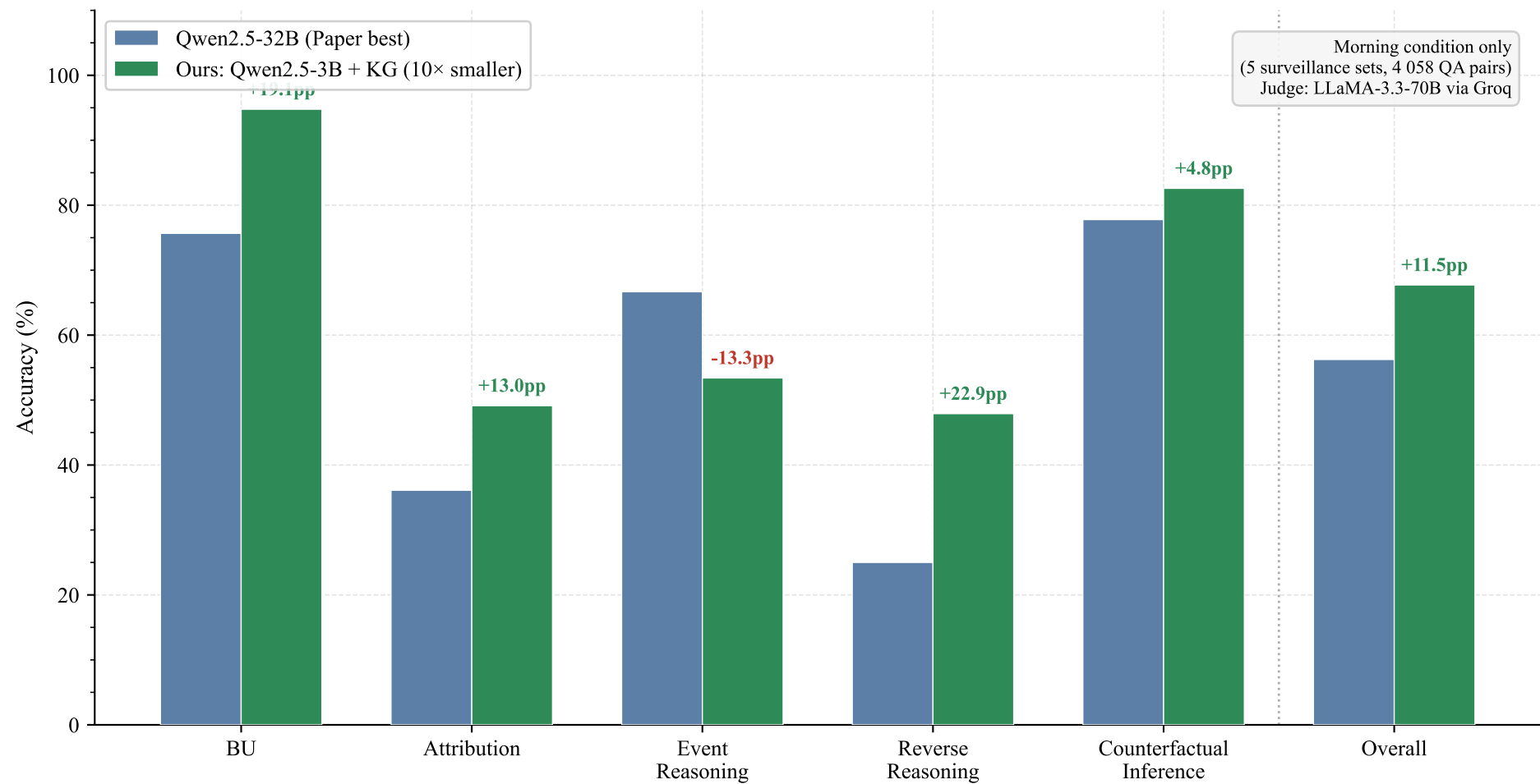
Figure 1 | Per-Category Accuracy: KG-Augmented Qwen2.5-3B vs. Paper Baseline
