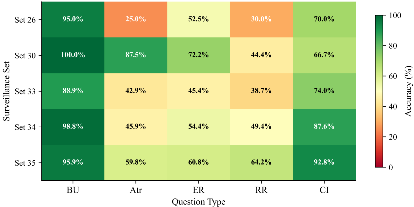
Figure 3 | Per-Set Accuracy Heatmap — KG-Augmented Qwen2.5-3B
