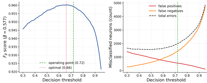
Fig. 2. Threshold analysis on the held-out test split. Left: F_\beta ( \beta=0.577 ) versus decision threshold, with the deployed operating point (0.72) and the F_\beta optimum (0.666) marked. Right: false positives, false negatives, and total errors versus threshold.
