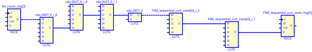
Figure 5.2: Post-synthesis critical path
