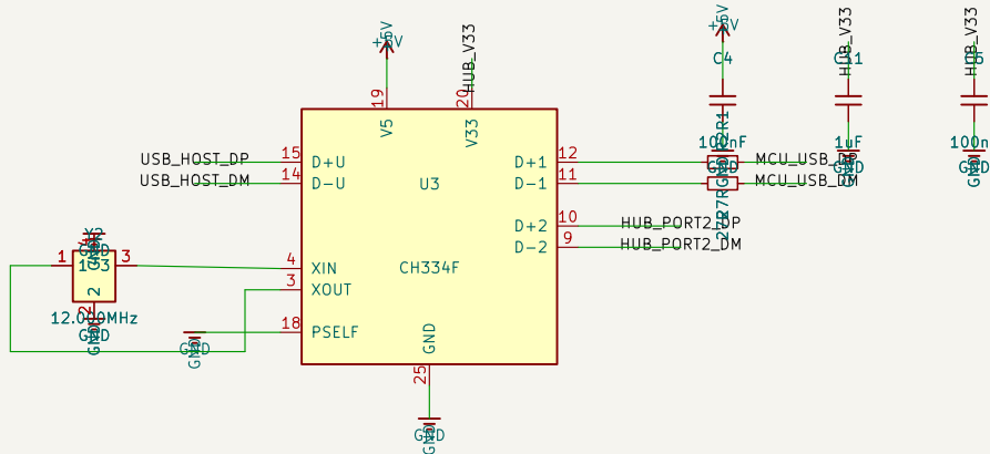
BLOCK 3: USB 2.0 HIGH-SPEED HUB (CH334F)
