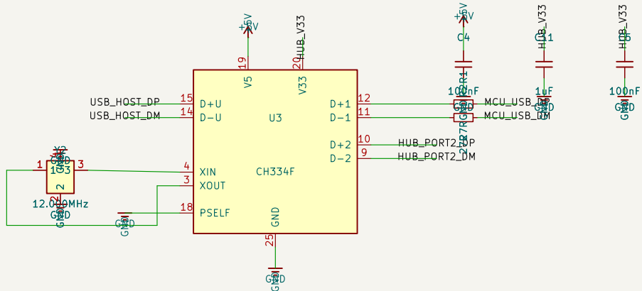
BLOCK 3: USB 2.0 HIGH-SPEED HUB (CH334F)
