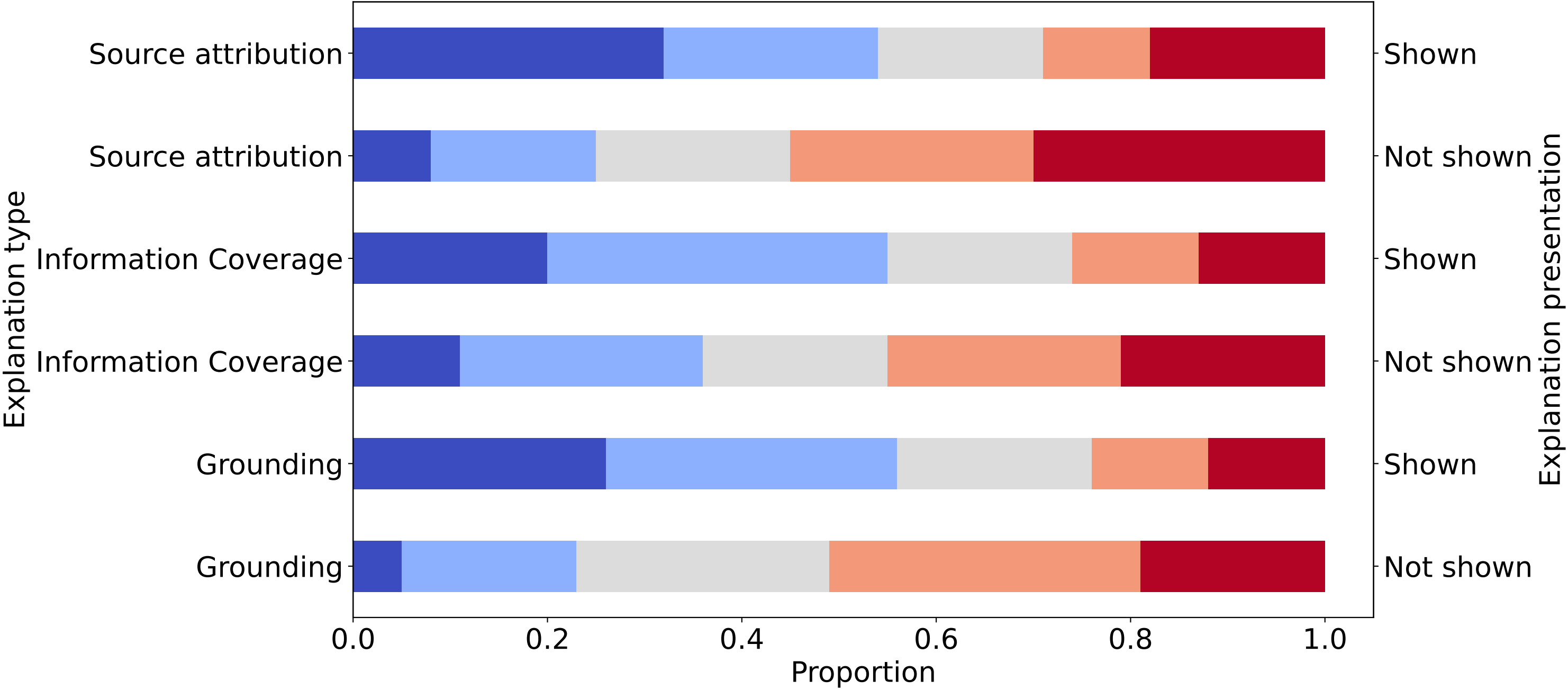
Distribution of Trust Scores
