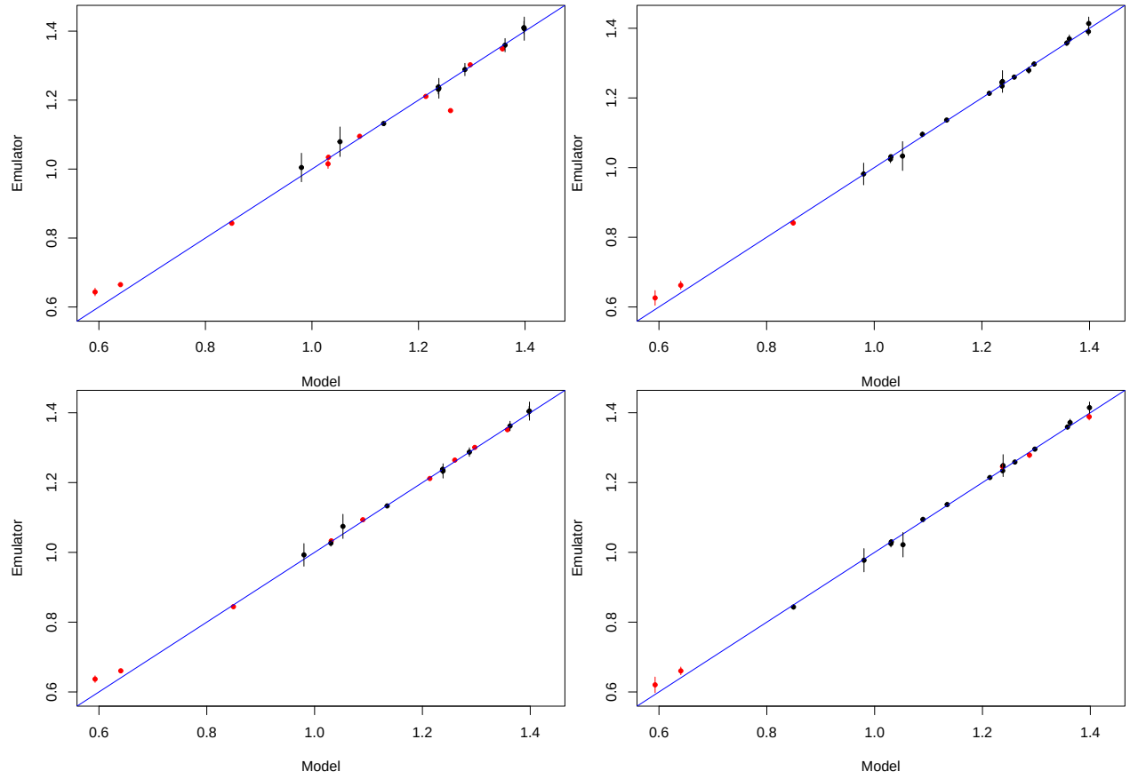
Figure 3: LOO cross validation. Top: Maximum likelihood estimation for the Gauss (left) and Matern 5/2 (right) kernels. Bottom: Marginal posterior mode estimation.
