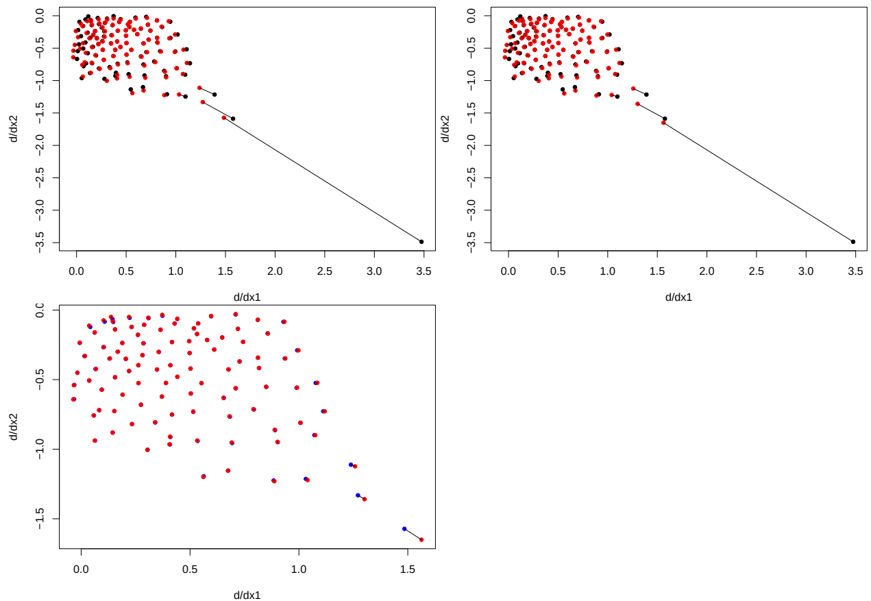
Figure 11: Top row: The estimated partial derivatives found by each estimation method (red dots, left MLE and right MAP) match the true partial derivatives (black) well. Bottom plot: The estimated partial derivatives returned by each estimation method are similar (blue for MLE and red for MAP).
