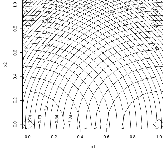
Figure 12: Contour plots for the functions y = \sqrt{2 - x_1^2 - x_2^2} and f(x_1, x_2) = \sqrt{2 - (x_1 - 1)^2 - x_2^2} .
