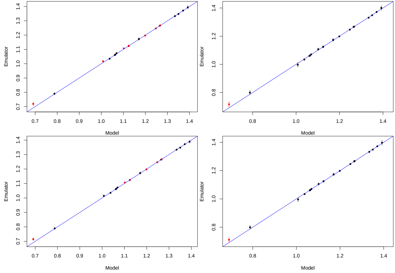
Figure 9: LOO cross validation. Top: Maximum likelihood estimation for the Gauss (left) and Matern 5/2 (right) kernels. Bottom: Marginal posterior mode estimation for the Gauss (left) and Matern 5/2 (right) kernels.
