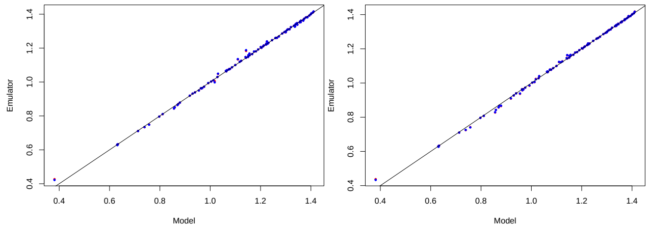
Figure 2: Emulator versus model for the new points. Left: Using a Gauss kernel. Right: Using a Matern 5/2 kernel. Red: MLE. Blue: MAP
