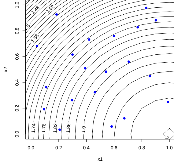
Figure 7: Contour plot for the function y = \sqrt{2 - (x_1 - 1)^2 - x_2^2} , with the location in the 2D input space of the observations' input settings shown in blue.
