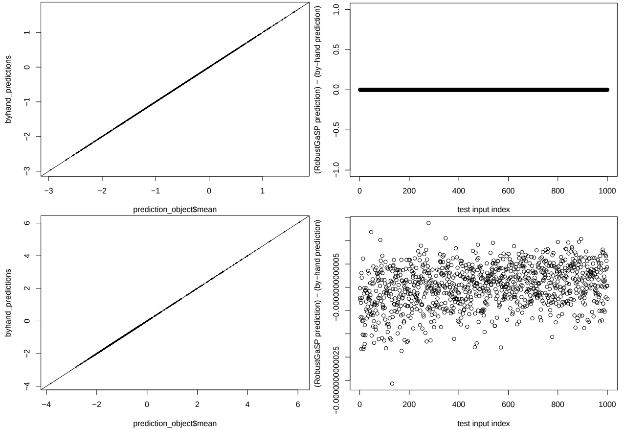
Figure 2: The predictions found by-hand match well with those made by both estimation methods (left), with the latter minus the former found to be essentially zero (right). Top: MLE. Bottom: MAP.
