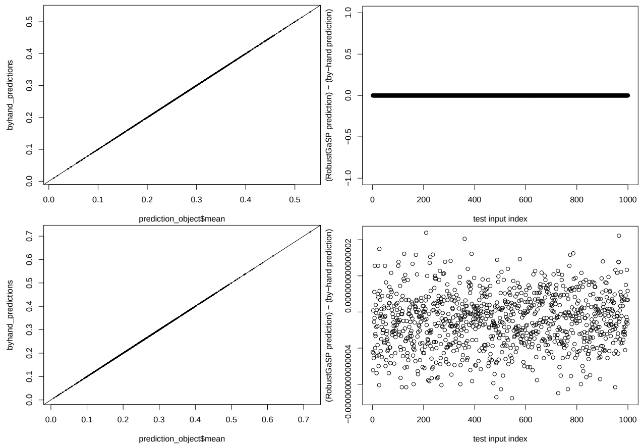
Figure 1: The predictions found by-hand match well with those made by both estimation methods (left), with the latter minus the former found to be essentially zero (right). Top: MLE. Bottom: MAP.
