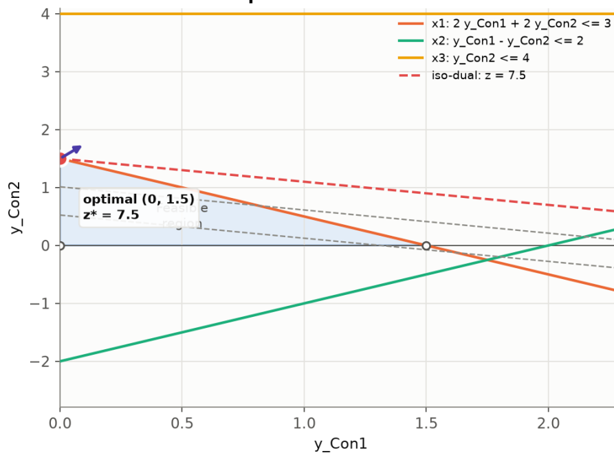
Graphical view of the dual
