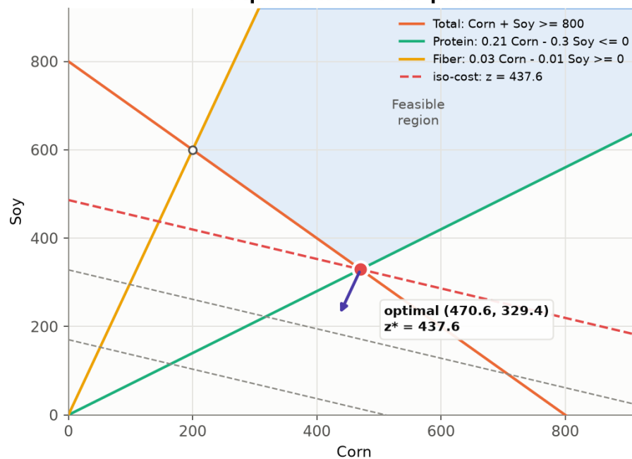
Graphical view of the primal
