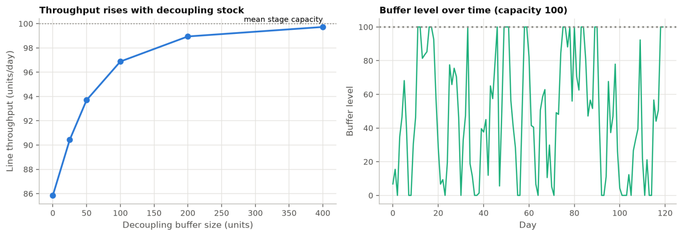
Figure 1.1 — Two-stage line simulation.
