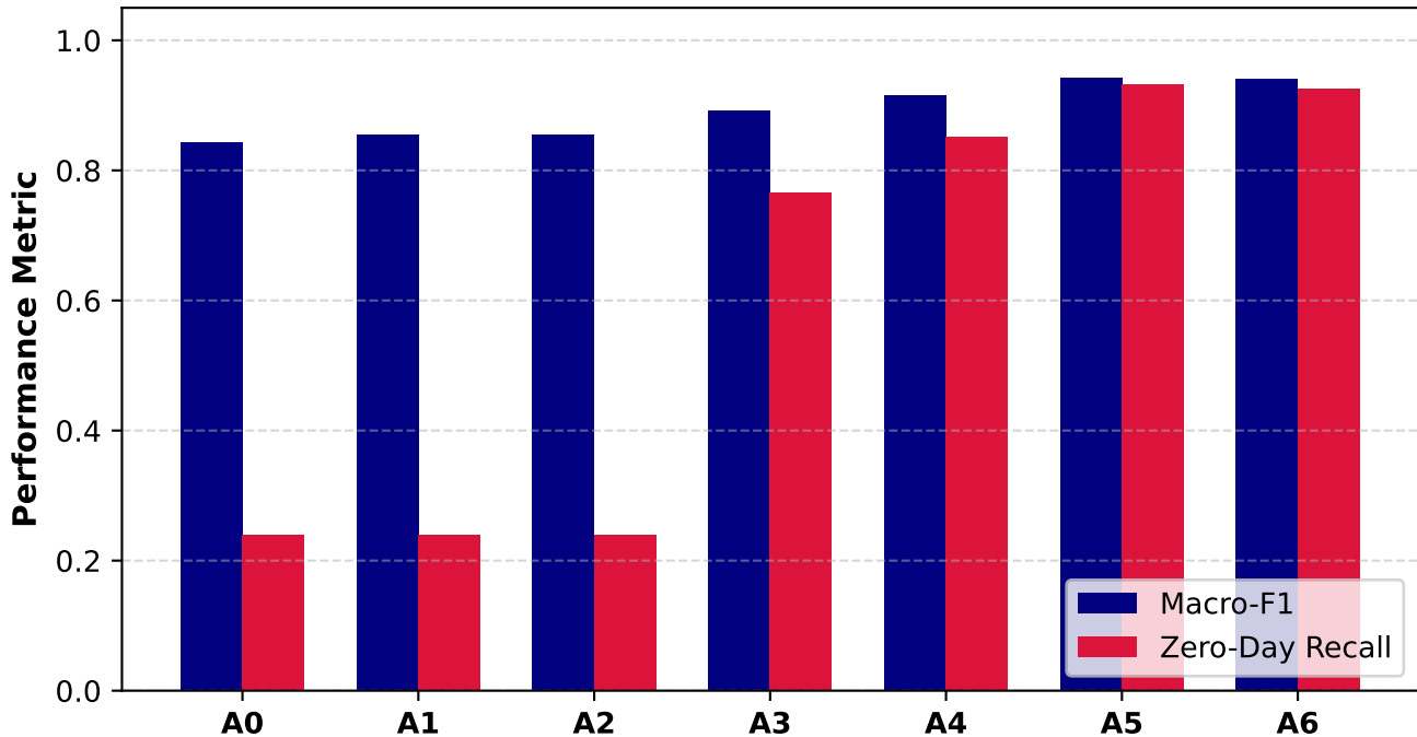
Architectural Ablation Ladder (A0 to A6)
