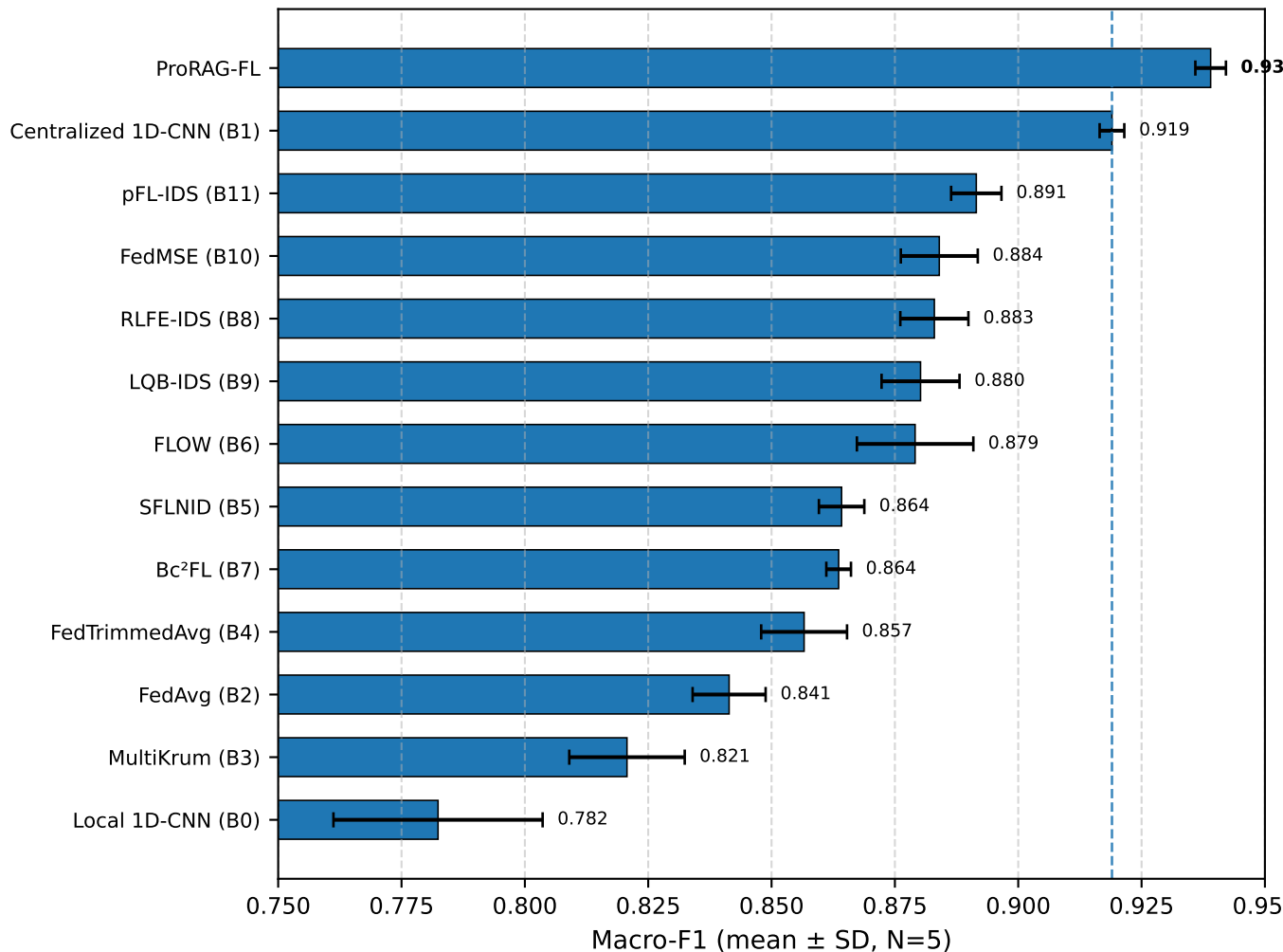
Known-Attack Macro-F1 Across Baselines
