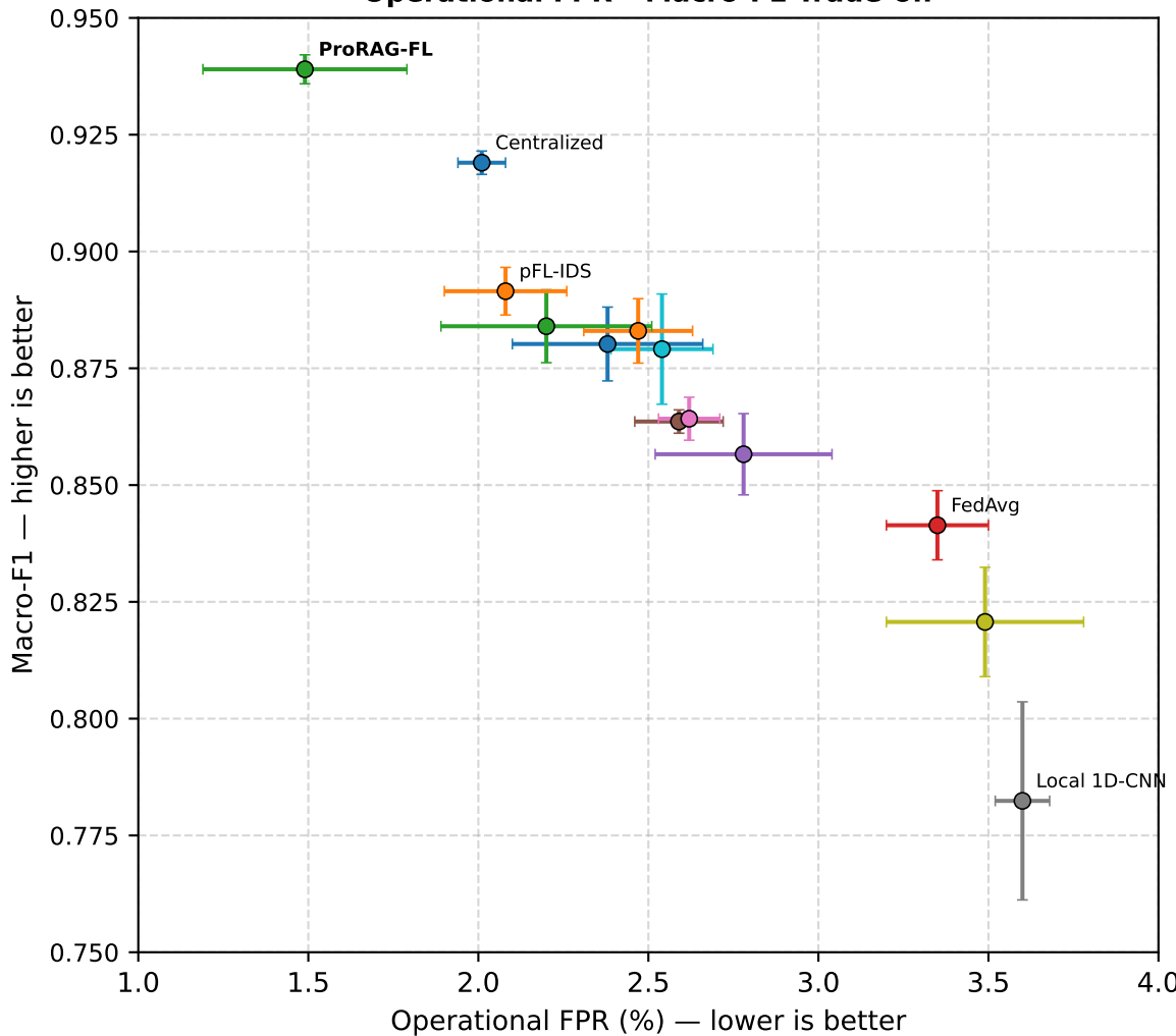
Operational FPR - Macro-F1 Trade-off
