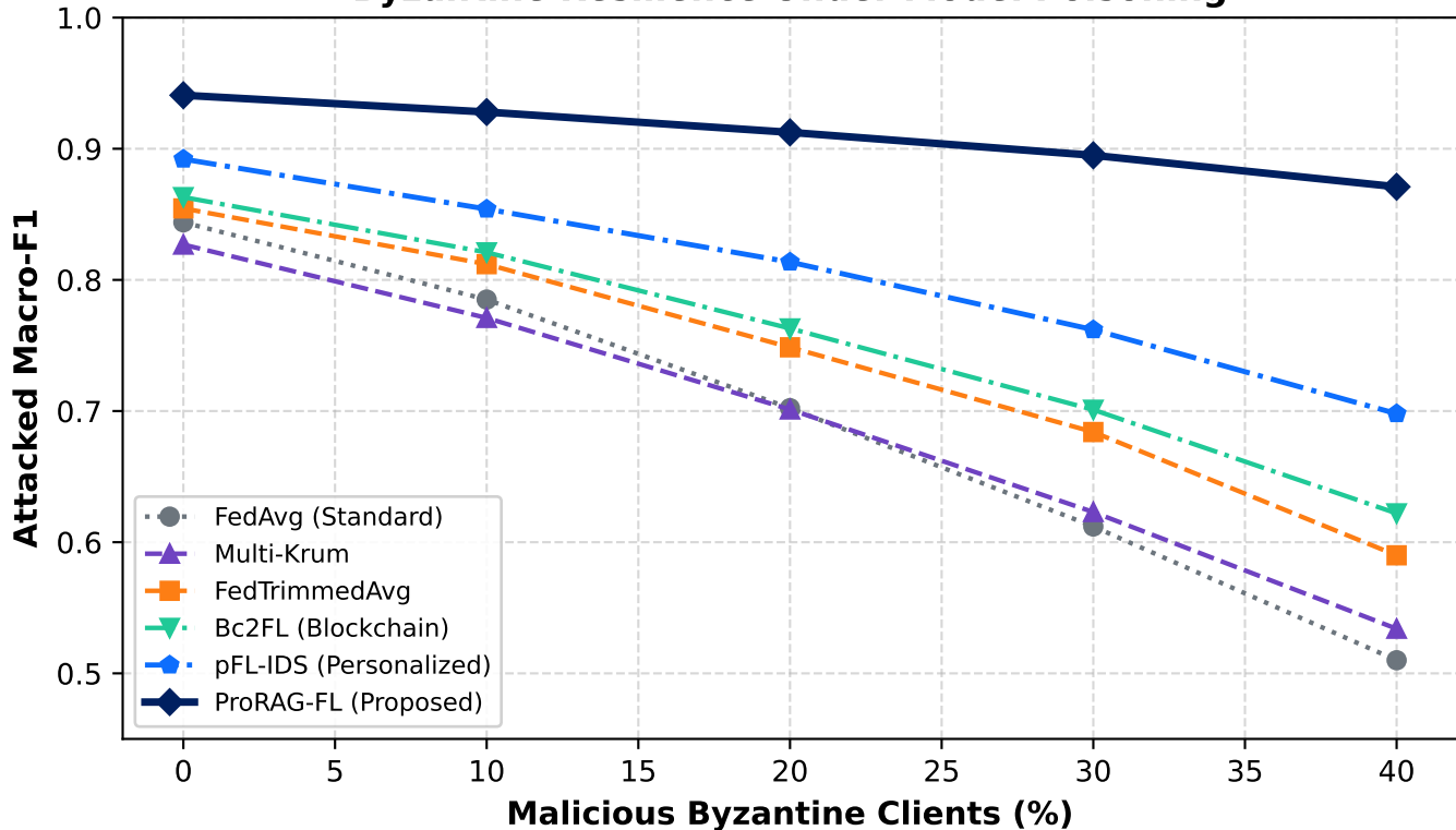
Byzantine Resilience Under Model Poisoning
