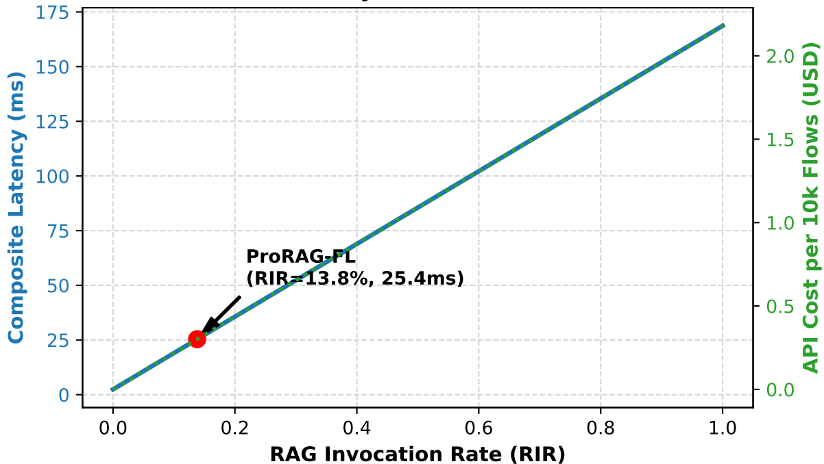
End-to-End Latency and Financial Cost vs. RIR
