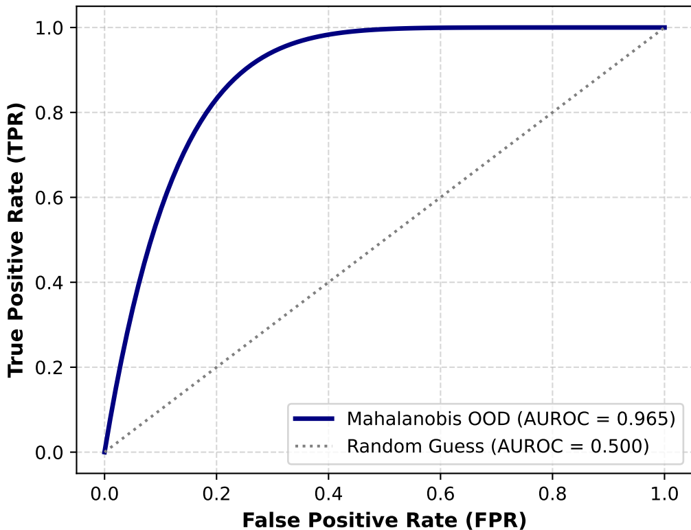
OOD Detection ROC Curve (Mahalanobis Distance)
