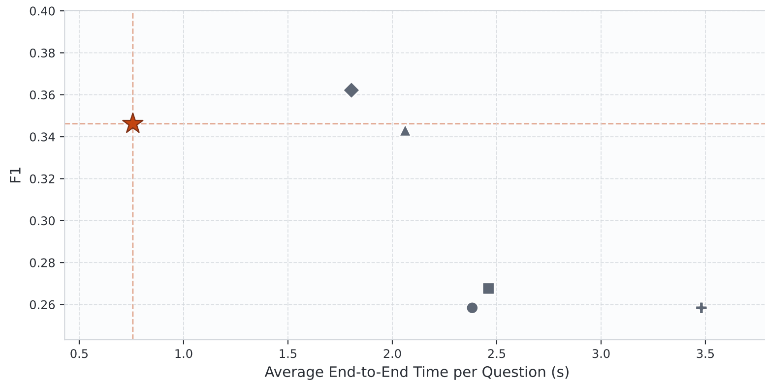
BERT (ONNX)
