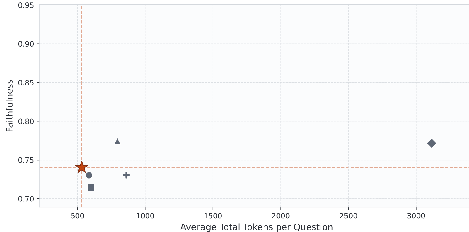
BERT (ONNX)
