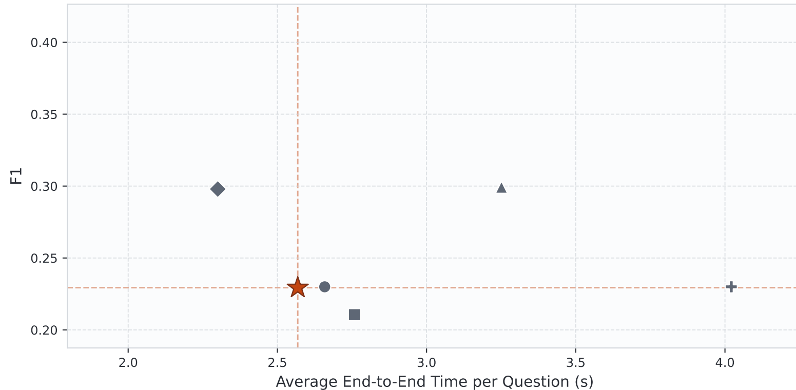
BERT (ONNX)
