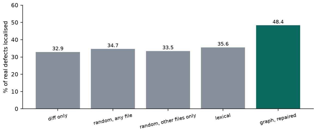
Figure 3. c-CRAB: real test-verified defects, five conditions run on one day with one pipeline, model and budget; 219 defects for the first four conditions and 218 for the random-other-files control.
