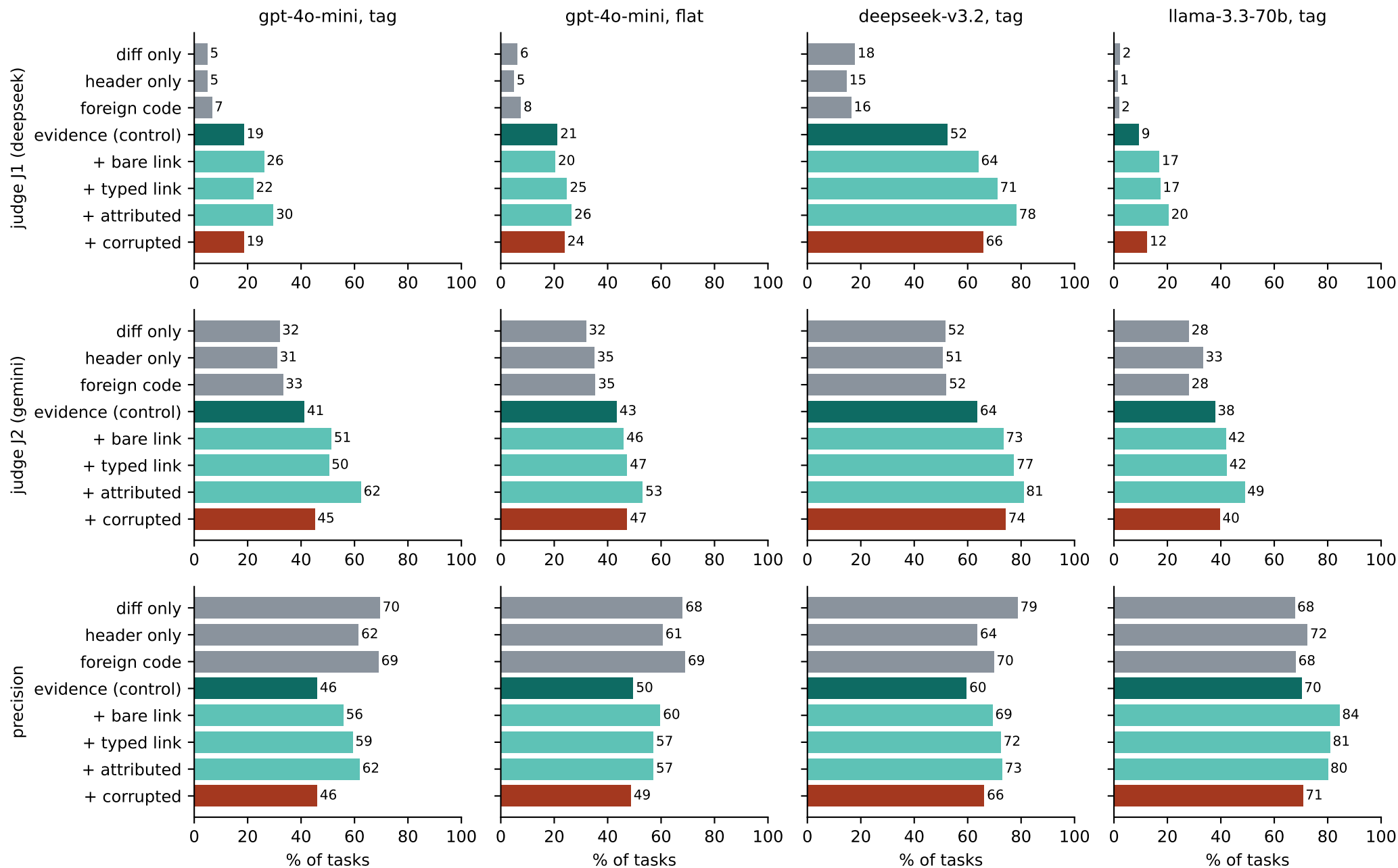
Figure 1. Per-arm rates on the rebuilt benchmark (225-230 paired defects per run). Arms 2-6 see identical snippets.
