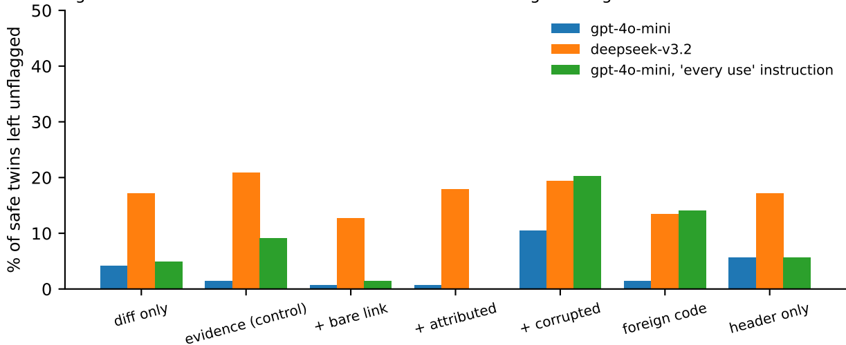
Figure 4. Safe twins: how often the model declines to flag a change the shown caller tolerates.
