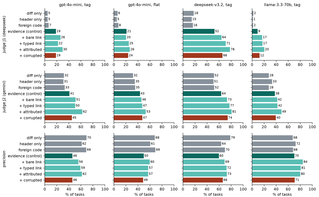
Figure 1. Per-arm rates on the rebuilt benchmark, four runs, three metrics. Arms 2–6 see identical snippets; only the metadata block differs.
