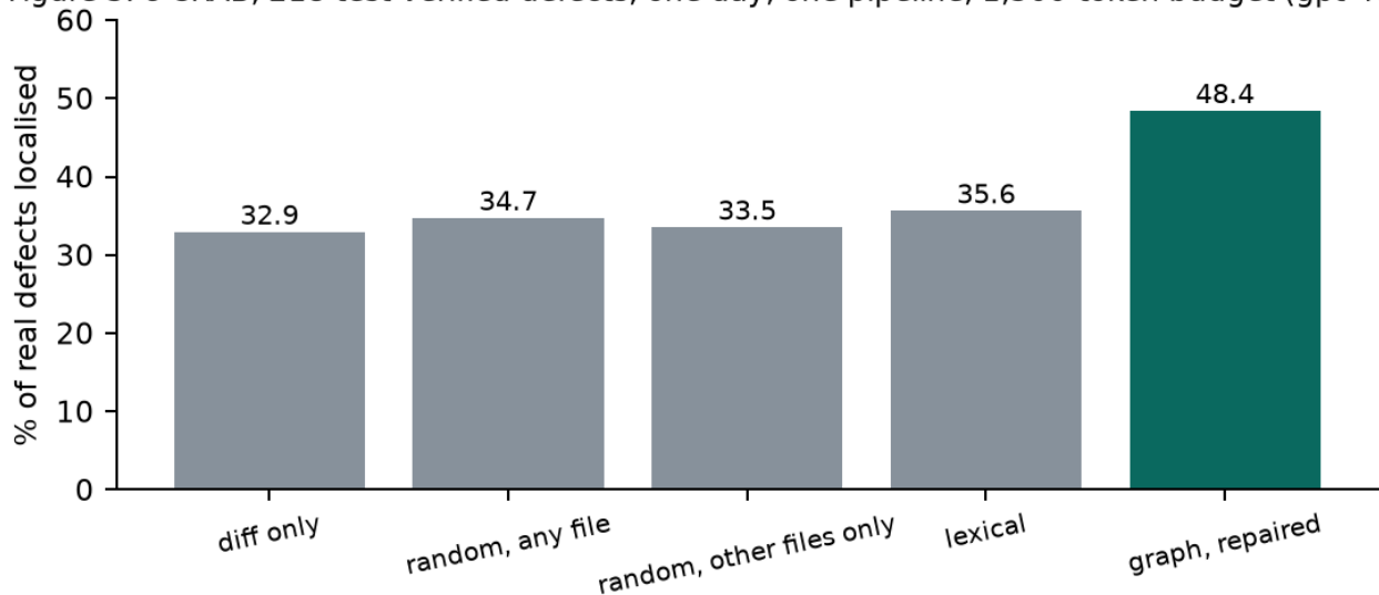
Figure 3. c-CRAB, 218 test-verified defects, one day, one pipeline, 1,500-token budget (gpt-4o-l)
