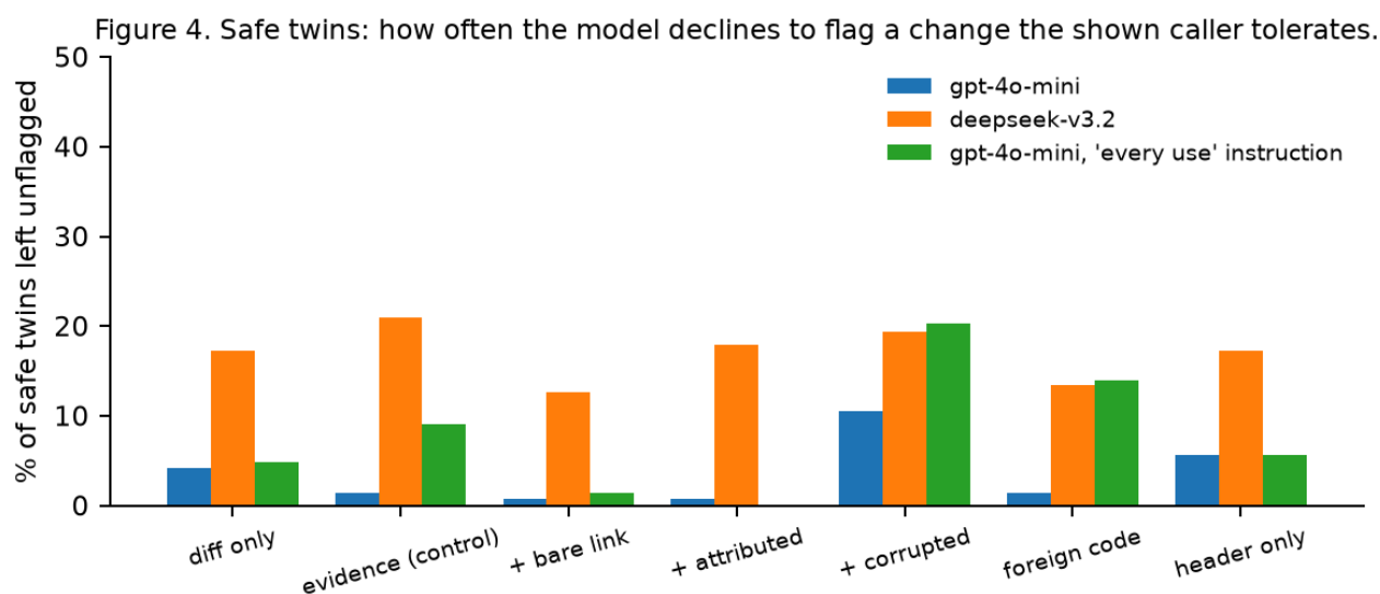
Figure 4. Safe twins: the share the model leaves unflagged, by arm, on two models and under the authoritative-callers instruction.
