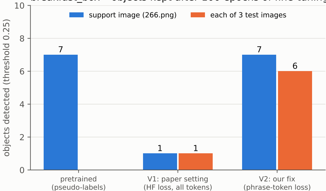
breakfast_box - objects kept after 100 epochs of fine-tuning
