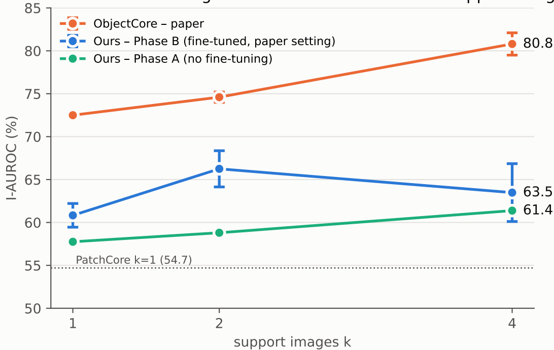
MVTec LOCO - image-level AUROC vs number of support images
