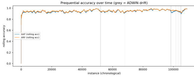
Figure 5: Prequential accuracy over the chronological stream for HAT and ARF; grey lines mark ADWIN-detected drift points.
