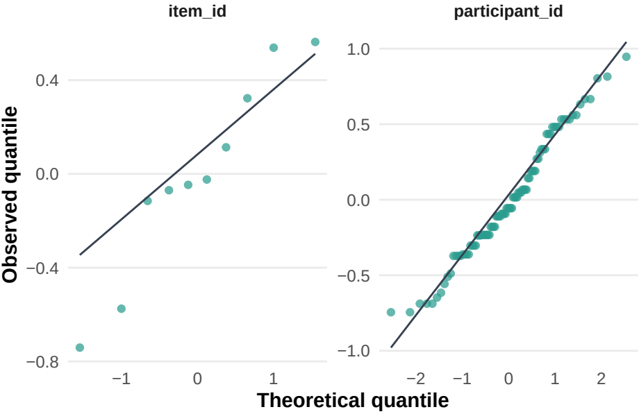
Random-intercept Q-Q plots
