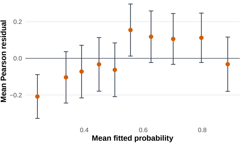
Binned Pearson residuals
