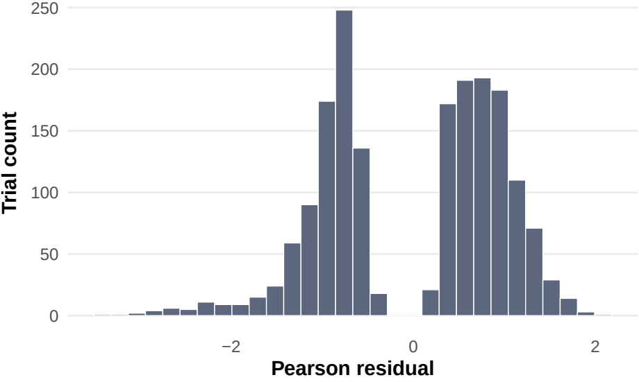
Pearson residual distribution
