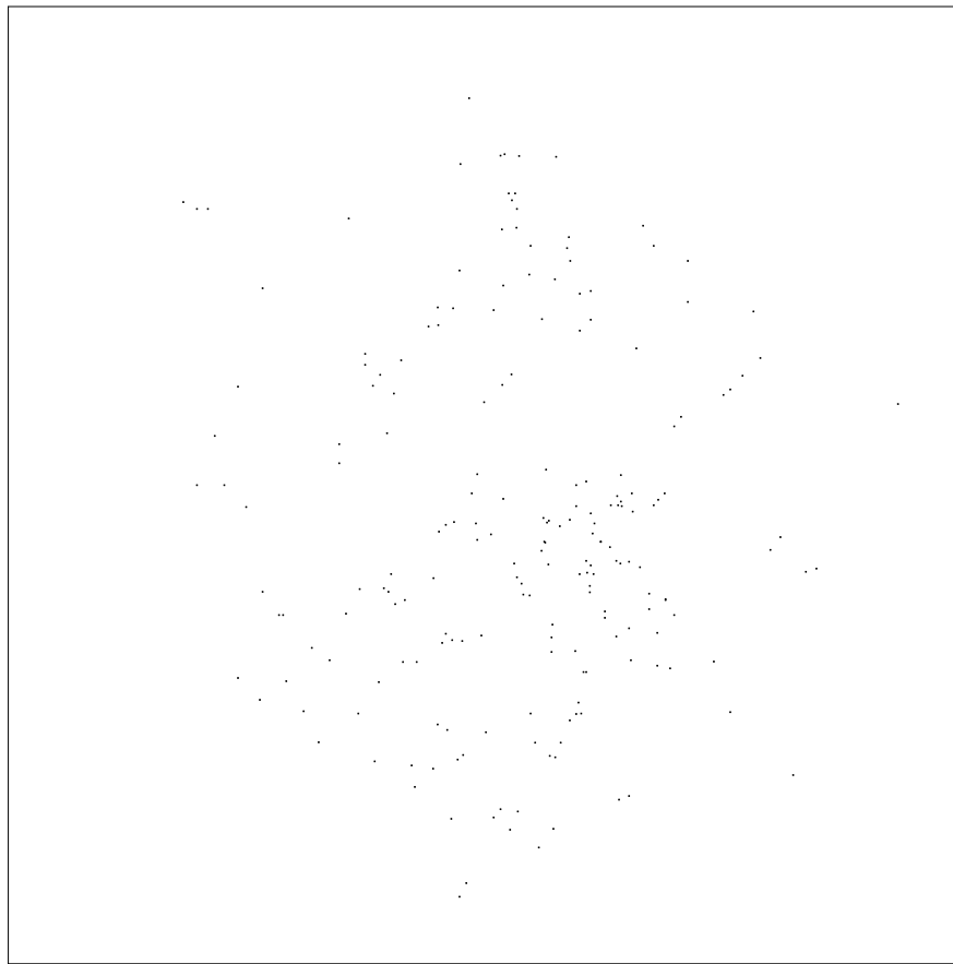
Drill Map: · 0.100mm / 0.0039" (202 holes)
