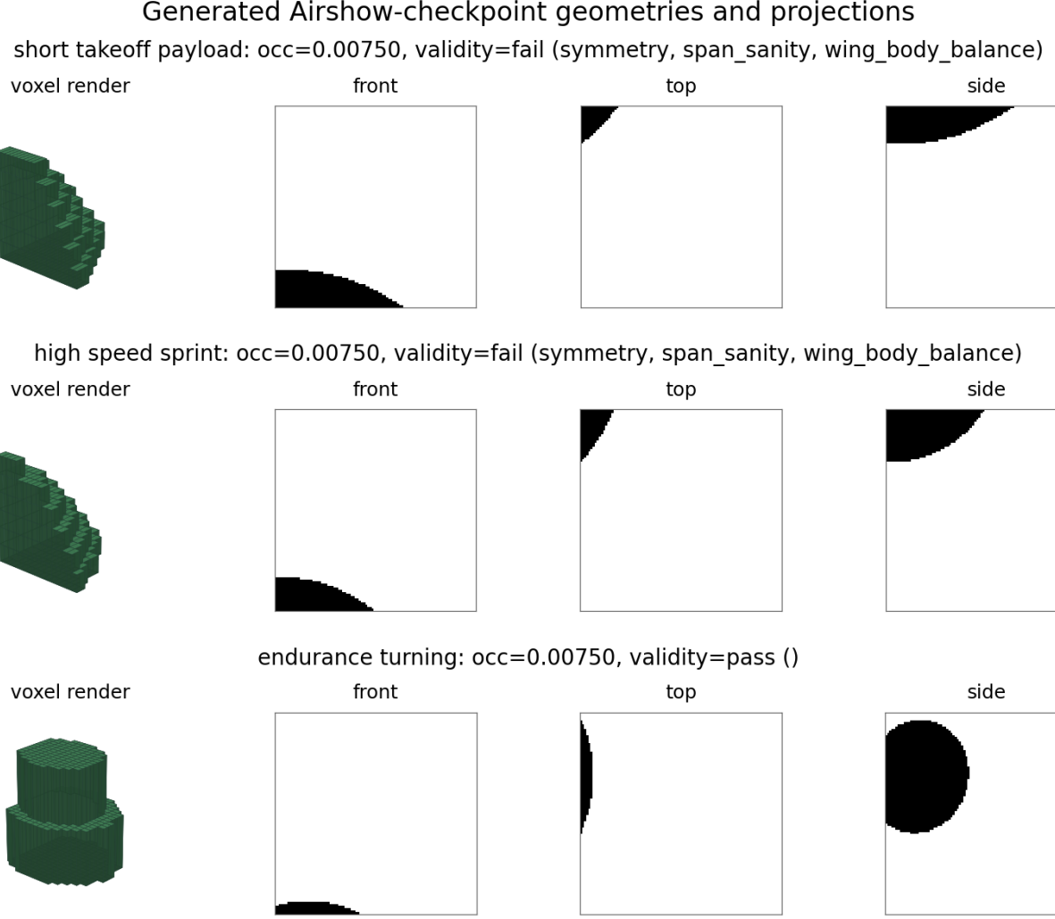
Fig. 10. Calibrated 96^3 coordinate-decoder geometries and projections. The figure documents the best high-resolution smoke result, including the two failing cases, rather than upgrading the result to a reliable aircraft-generation claim.
