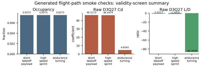
Fig. 9. Calibrated 96^3 top-k flight-path metrics at 0.75% occupancy. One case passes the heuristic aircraft-validity screen, while two still fail shape checks; all CFD quantities remain internal non-claim-bearing D3Q27 smoke outputs.
