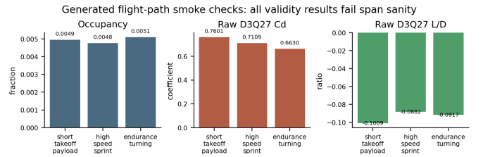
Fig. 7. Raw 32^3 generated flight-path metrics. The generated artifacts have finite internal D3Q27 outputs, but all still fail aircraft-validity gates and therefore remain non-claim-bearing.
