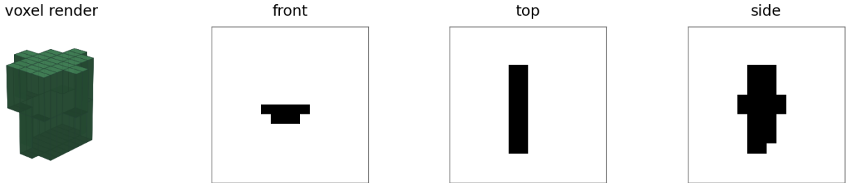
Fig. 6. Generated Airshow-checkpoint voxel geometries and orthographic occupancy projections for the three conditioned smoke cases. The visualized artifacts are intentionally shown despite failing span_sanity: they demonstrate nonempty generation and exportable grids, while also showing why the current checkpoint should not be described as producing valid aircraft.
