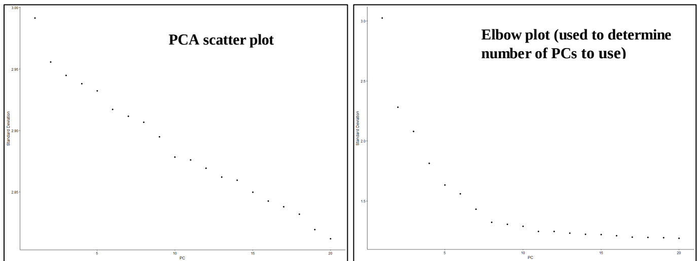
Figure 3 – PCA diagnostics
