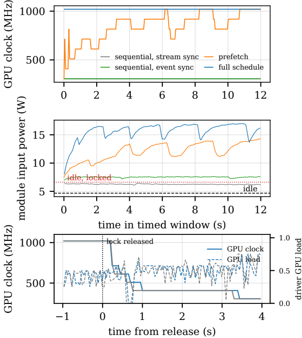
Figure 3: GPU clock (top) and module input power (middle) during the first 12 s of four YOLO26n application runs on val2017 under default governors (20 Hz samples); the two sequential traces coincide at 306 MHz in the top panel. Bottom: the lock-then-release experiment. The sequential pipeline is started with the GPU clock locked at 1020 MHz, and the lock is released at t=0 (dotted line). Clock (solid) and driver GPU load (dashed, right axis) of two repeats fall to the 306 MHz floor within about 3.4 s.
