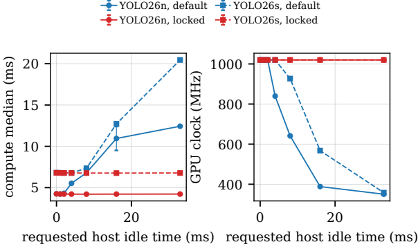
Figure 1: Median GPU compute time of the uint8 FP16 engines in trtexec (left) and mean sampled GPU clock (right) versus a forced idle gap between inferences. Mean of two 15s runs per point. Default governors (blue) versus jetson_clocks (red). The gap is host idle time ( -idleTime ), not a frame period.
