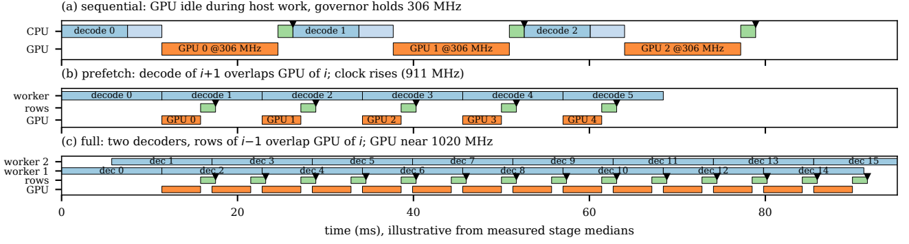
Figure 4: Schematic of the three schedules. The time axis uses the measured stage medians of the sequential float pipeline of Section 5: decode 7.5 ms, letterbox 3.9 ms, rows \approx 1.5 ms and engine 13.2 ms (host-measured enqueue-to-completion at 306 MHz; the device-side CUDA-event share is 12.5 ms, Table 5). The stage medians sum to 26.0 ms, while the measured period is 29.5 ms (33.9 images/s). The difference is per-image main-thread work outside the timed stages. Markers (▼) show when each frame's detections become ready. The bars show the structure, not the measured throughputs. In (a) every host stage is GPU idle time, so the governor holds the minimum clock. In (b) and (c) the host stages overlap engine execution.
