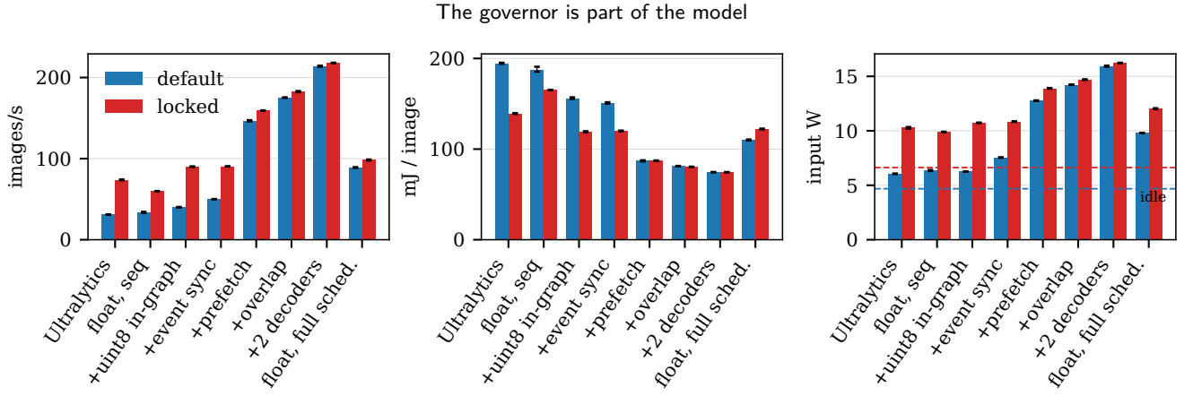
Figure 5: Throughput, energy per image and mean input power along the ladder of Table 6 (bars: mean; whiskers: minimum-maximum of three runs). Dashed lines in the right panel mark idle input power (4.68 W default, 6.62 W locked).
