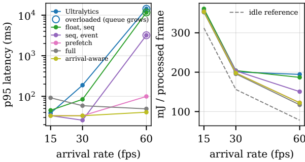
Figure 6: Streaming at 15, 30 and 60 fps under default governors. Left: p95 latency from frame release to finished rows (log scale). Open markers denote overloaded cells (processed rate below arrivals), whose latency reflects a queue growing over the finite run, not a steady state. Right: module input energy per processed frame (the denominator when a pipeline is overloaded). The dashed line is idle power divided by the frame rate.
