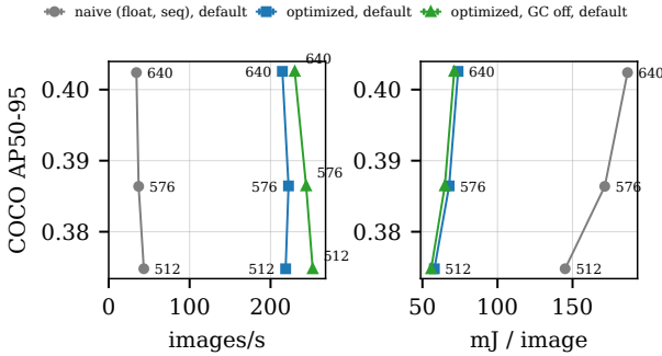
Figure 7: COCO val2017 AP against throughput (images/s) and energy per image (mJ) for static 512/576/640 YOLO26n engines, default governors, mean of two runs (whiskers: repeat min/max; labels: input size). In the full pipeline (squares), lower resolution buys only 2–4% throughput because the pipeline is limited by the main thread, not by GPU throughput; the GPU already runs at its maximum clock. Disabling CPython’s cyclic GC (triangles, identical predictions) raises all three points and widens the spread to 6–10%.
