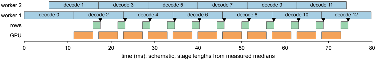
(c) Full: two decode workers; rows of frame i-1 overlap the engine of frame i ; GPU near 1020 MHz
