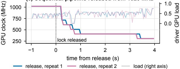
(c) Sequential pipeline released from 1020 MHz
