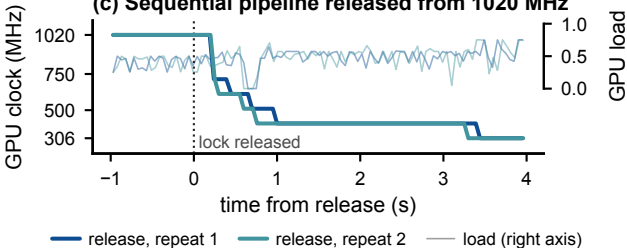
(c) Sequential pipeline released from 1020 MHz
