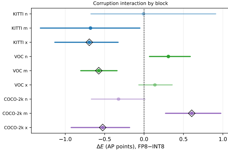
Figure 2: Paired corruption interaction \Delta E (FP8-INT8) with 95% common-image-bootstrap intervals. Solid markers denote intervals excluding zero (unadjusted); open diamonds mark blocks surviving Holm adjustment across the nine blocks ( p_{\text{Holm}} < 0.05 ). The sign reverses across dataset×model blocks, so the interaction cannot be summarized as a single format-level effect.
