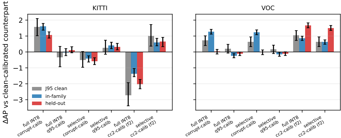
Figure 4: Calibration variants versus their clean-calibrated counterparts (AP points, 95% paired-bootstrap intervals). Grey: J95 clean control; blue: in-family corruptions; red: held-out corruptions. The family roles swap between folds: fold 1 calibrates Gaussian noise and JPEG and holds out fog and motion blur, while the groups marked “f2” (fold 2) calibrate fog and motion blur and hold out Gaussian noise and JPEG; for the q95-calibration rows, which see no corrupted images at all, the in-family/held-out labels only mark the evaluation partition. On KITTI fold 1 and the KITTI fold-2 full-INT8 tier the clean and held-out bars move together—the fold-2 full-tier movement being a harm, not a gain—so those held-out changes are not corruption-specific (the KITTI fold-2 selective tier instead improves significantly on both bases); VOC fold 1 moves the in-family and clean bars but leaves held-out null, and the VOC fold-2 groups are the exceptions, where held-out clearly exceeds clean for both the full and the selective tier. Codec-only calibration (q95-calib) shifts the full-INT8 arm’s aggregate bases by less than half an AP point; at per-cell granularity it moves individual cells significantly in both directions (a gain on the saturated KITTI motion-blur-s5 wall, a loss on a VOC noise cell, and several gains on the KITTI selective tier), so codec adaptation is real even where its aggregate contribution is small—a codec effect on shared failure cells rather than evidence of corruption coverage.
