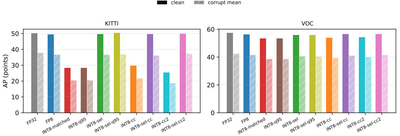
Figure 3: RetinaNet recipe arms on KITTI and VOC: clean AP versus 12-cell corruption mean. INT8-matched collapses on KITTI (dataset-dependent); selective precision (INT8-sel = INT8-selective, reg-head in floating point) restores FP8-level behavior on KITTI and leaves a small residual on VOC; the calibration variants (INT8-q95 = codec-only calibration; INT8-cc = fold-1 corruption-aware calibration on noise and JPEG; INT8-cc2 = fold-2 calibration on fog and motion blur; a “sel-” prefix marks the selective recipe with the regression head in floating point) shift the matched arm little.
