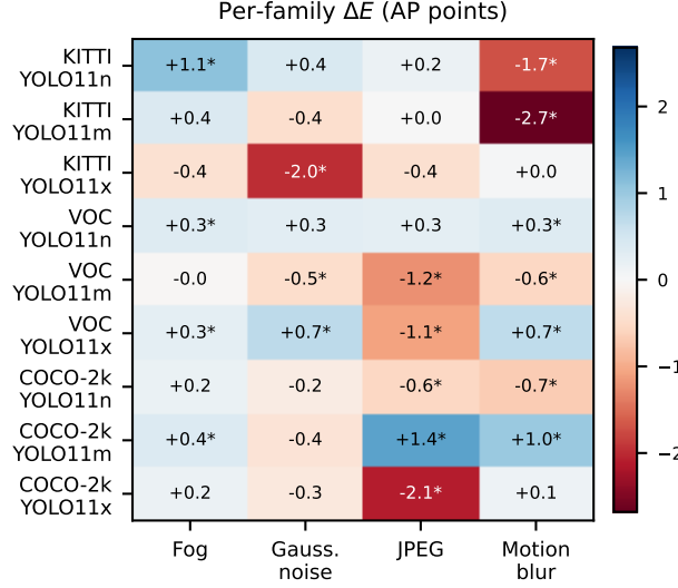
Figure 3: Per-family interaction \Delta E (FP8 minus INT8, on the J95-controlled basis) across the nine paired blocks, in AP points. Star: unadjusted 95% bootstrap interval excludes zero. Both signs occur inside every corruption family, and every block mixes signs across families—the heterogeneity quantified in the text.
