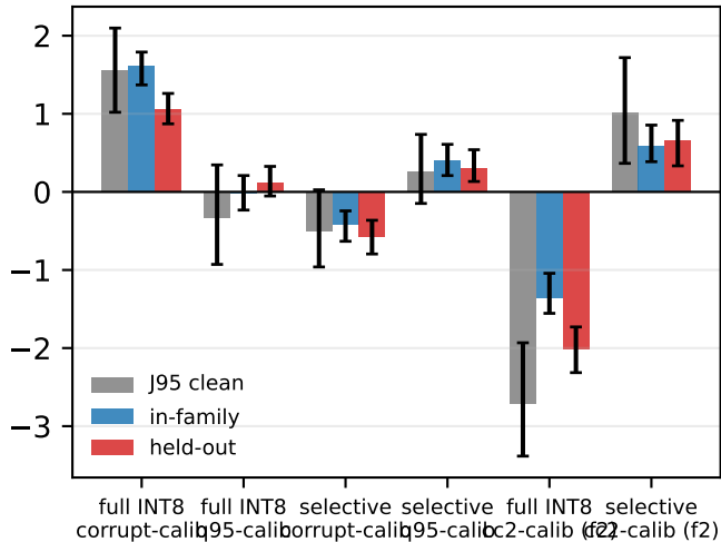
KITTI
