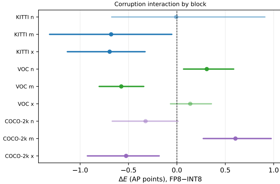
Figure 2: Paired corruption interaction \Delta E (FP8-INT8) with 95% common-image-bootstrap intervals. Solid markers denote intervals excluding zero. The sign reverses across dataset×model blocks, so the interaction cannot be summarized as a single format-level effect.
