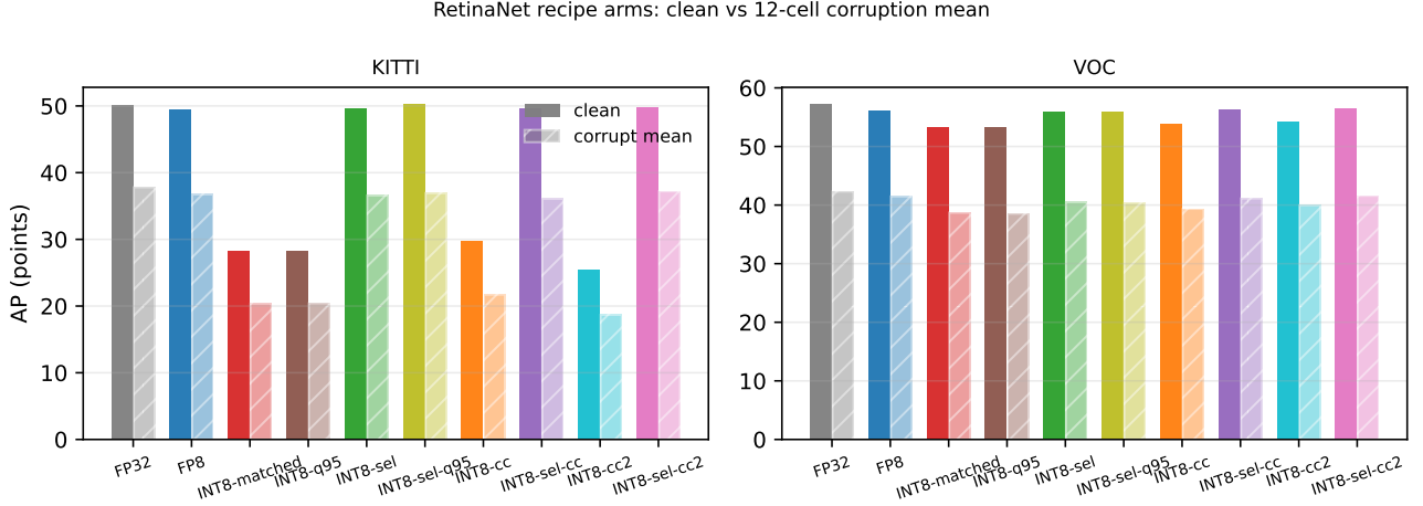
Figure 3: RetinaNet recipe arms on KITTI and VOC: clean AP versus 12-cell corruption mean. INT8-matched collapses on KITTI (dataset-dependent); selective precision (INT8-sel = INT8-selective, reg-head in floating point) restores FP8-level behavior on KITTI and leaves a small residual on VOC; the calibration variants (INT8-q95 = codec-only calibration; INT8-cc = fold-1 corruption-aware calibration on noise and JPEG; INT8-cc2 = fold-2 calibration on fog and motion blur; a “sel-” prefix marks the selective recipe with the regression head in floating point) shift the matched arm little.
