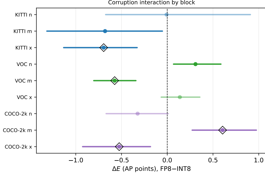
Figure 4: Paired corruption interaction \Delta E (FP8-INT8) with 95% common-image-bootstrap intervals. Solid markers denote intervals excluding zero (unadjusted); open diamonds mark blocks surviving Holm adjustment across the nine blocks ( p_{\text{Holm}} < 0.05 ). The sign reverses across dataset x model blocks, so the interaction cannot be summarized as a single format-level effect.
