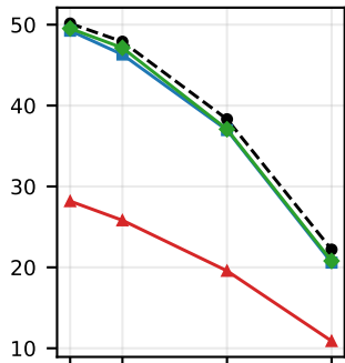
Gaussian noise
