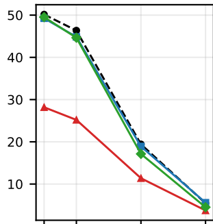
Motion blur
