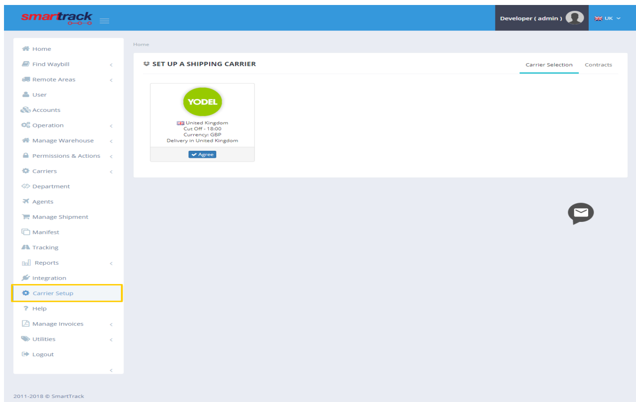
Figure 16-1 Carrier Setup
