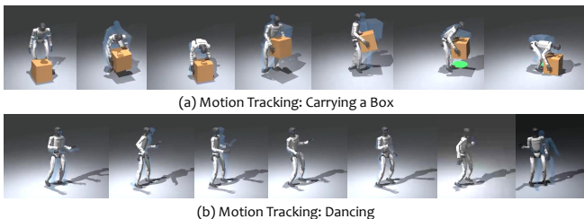
Fig. 7: Motion tracking with a unified policy. I-BFM tracks generated whole-body motions for both box carrying (top) and dancing (bottom). Translucent blue figures denote the reference motion.
